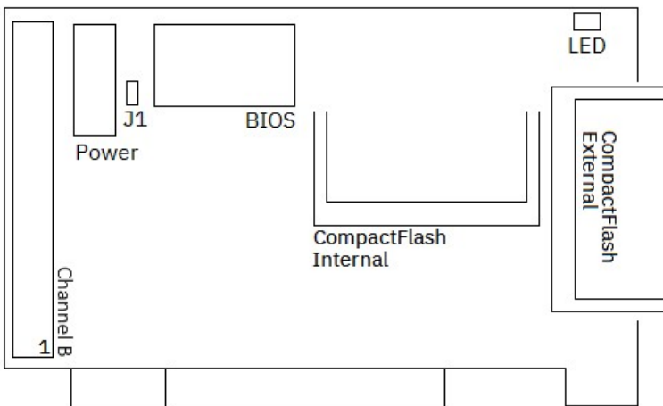
Figure 1 – Adapter layout
